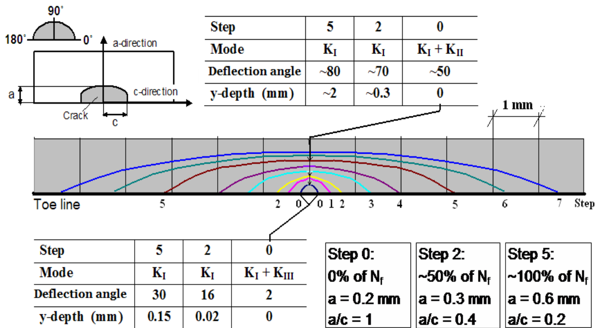
Figure 16. A top view of the crack shape of a 3D cold lap from start (step 0, a/c = 1 ) to approximately the end of life (step 7, a/c \approx 0.1 ).
