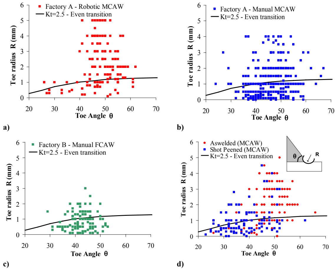
Figure 2. Local weld geometry: a) Factory A (Robotic MCAW); b) Factory A (Manual MCAW); c) Factory B (Manual FCAW); d) before and after shot peening.
