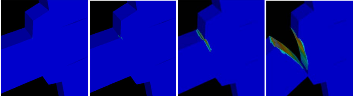
Figure 14. 3D-model of a cold lap having a/c=1 at start. Pictures show the state from start (left with a/c=1 ) to near failure (right with a/c\approx 0.1 ). Due to symmetry only half a cold lap is modelled.
