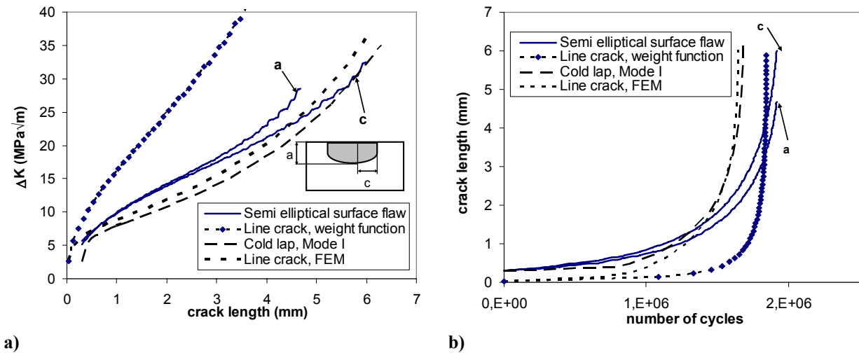
Figure 9. Behaviour of different crack shapes: a) stress intensity factors; b) fatigue life.
