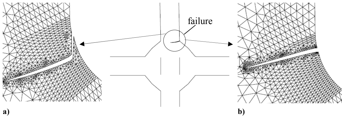
Figure 6. Simulation of fatigue crack propagation from: a) a cold lap (0.3 mm) and b) a straight-fronted line crack (0.03 mm).
