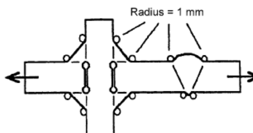
Figure 4. Fictitious rounding of weld toes and roots [8].
