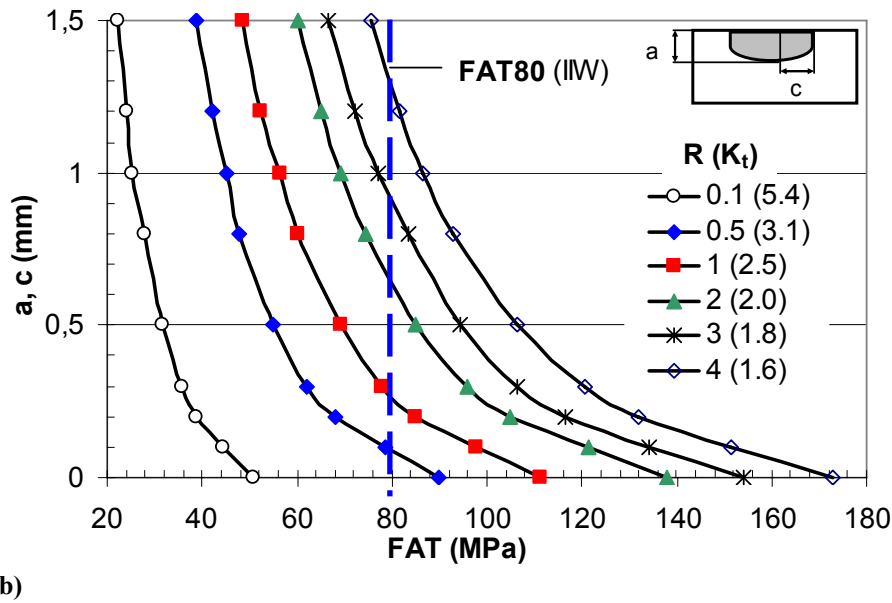
Figure 10. Fatigue strength (FAT) for different toe radius ( R ), stress concentration ( K_t ) and crack size: a) cold lap defect; b) semi elliptical surface flaw. The dashed lines indicate FAT values at K_t < K_{th} ( 2 \text{ MPa}\sqrt{\text{mm}} ).
