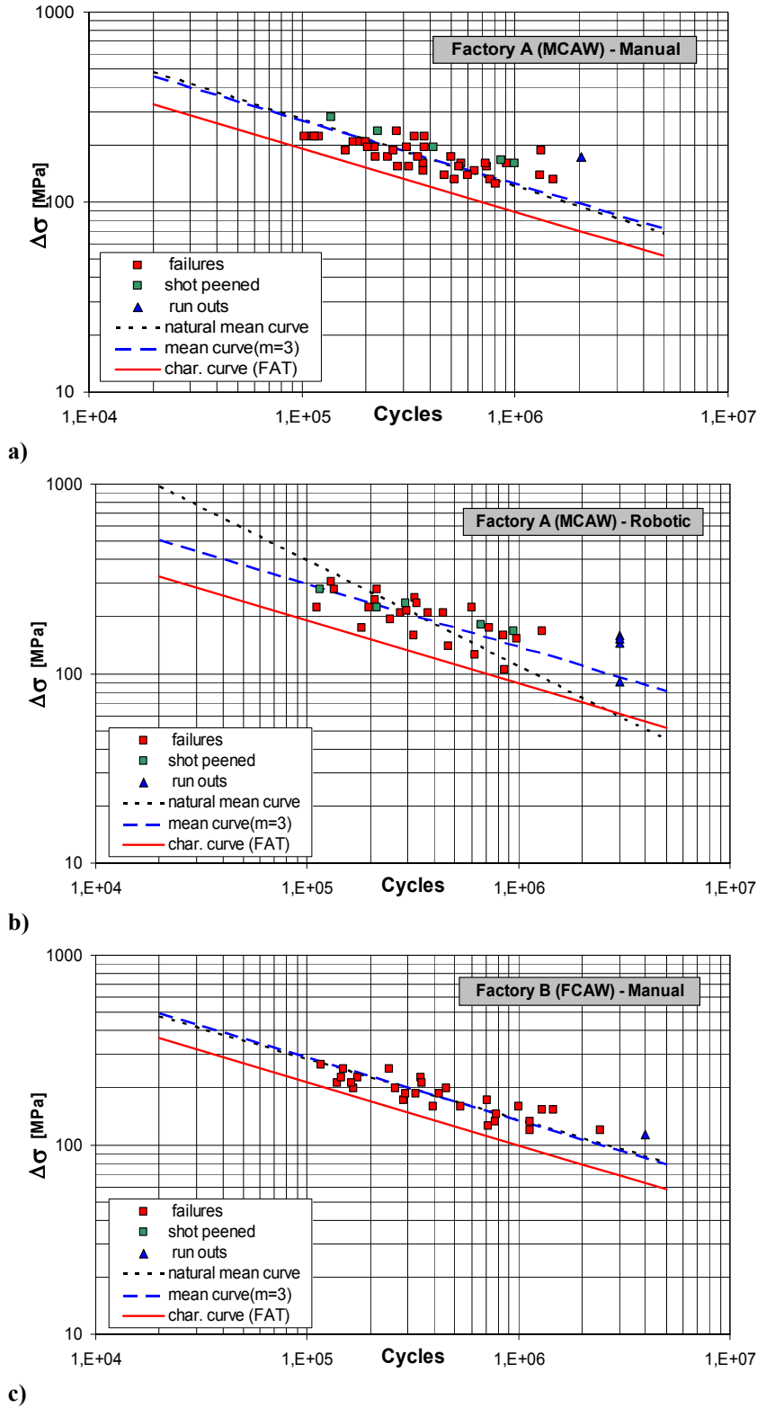
Figure 3. Fatigue test result compiled in S-N-curves: Factory A; (MCAW) a) manual; b) robotic, Factory B (FCAW); c) manual.
