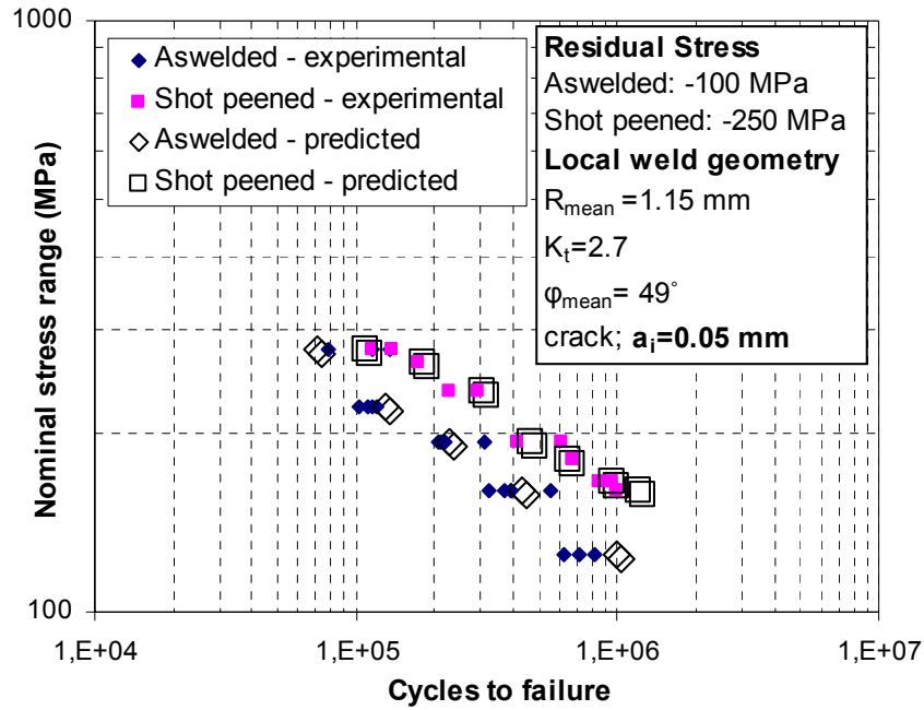
Figure 11. Predicted and experimentally obtained fatigue lives.
