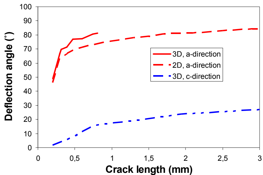
Figure 17. Comparison of deflection angles in 3D- and 2D LEFM-analysis of crack growth from spatter induced cold lap and line cold lap, respectively. Crack length is calculated using d_a + \text{depth} and d_c + \text{depth} , respectively.
